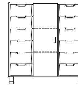
M 18 157 12 CASSETTE IN PLASTICA - 1 ANTA cm 104x41x114 H
